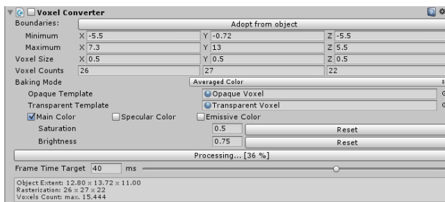
Voxel Converter shows the current progress
