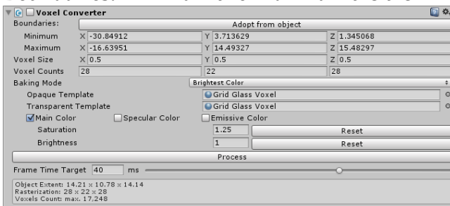
Voxel Converter inspector with all properties
