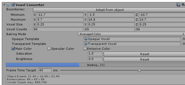
Voxel Converter inspector at runtime while processing
